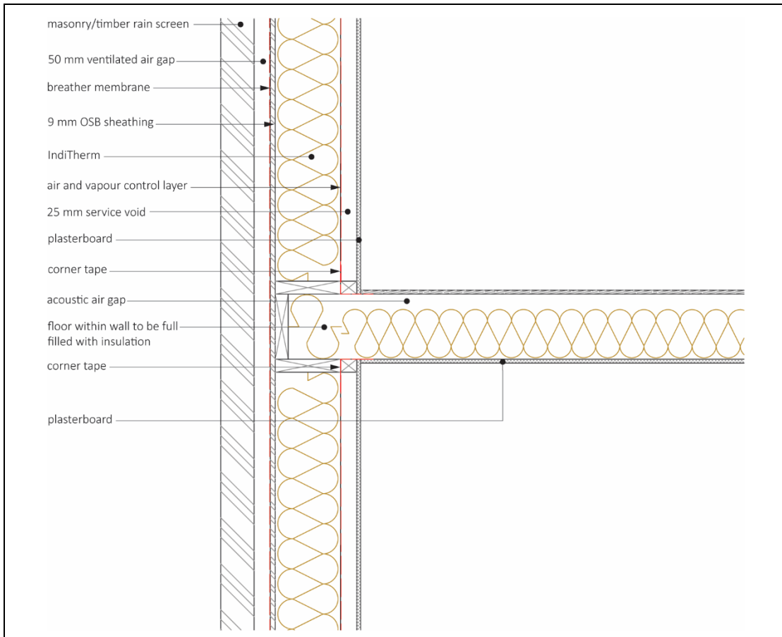
Figure 3 Wall to intermediate floor junction detail
